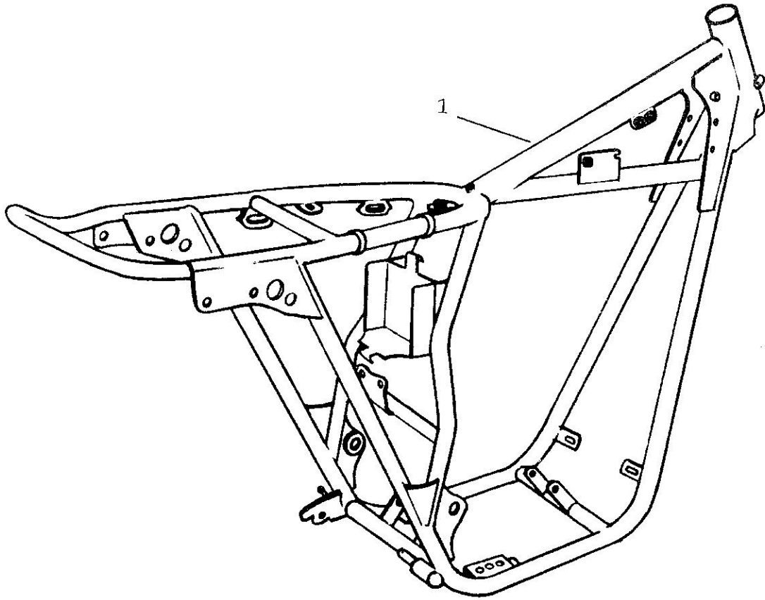
FRAME, CENTRAL
