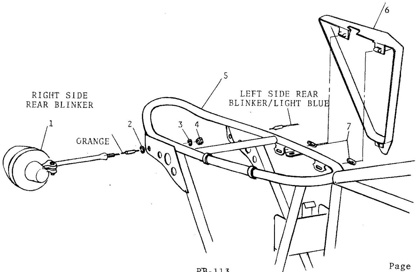
SIDE COVER & REAR TURN SIGNAL ASSEMBLY
